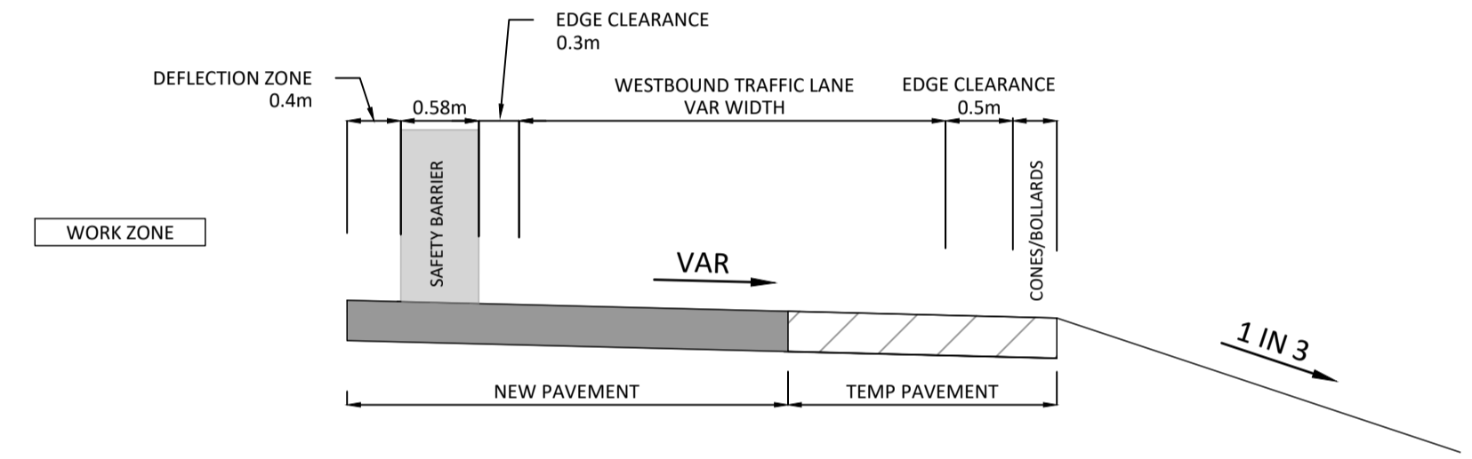
TYPICAL SECTION - TRAFFIC MANAGEMENT STAGE 3 NTS
