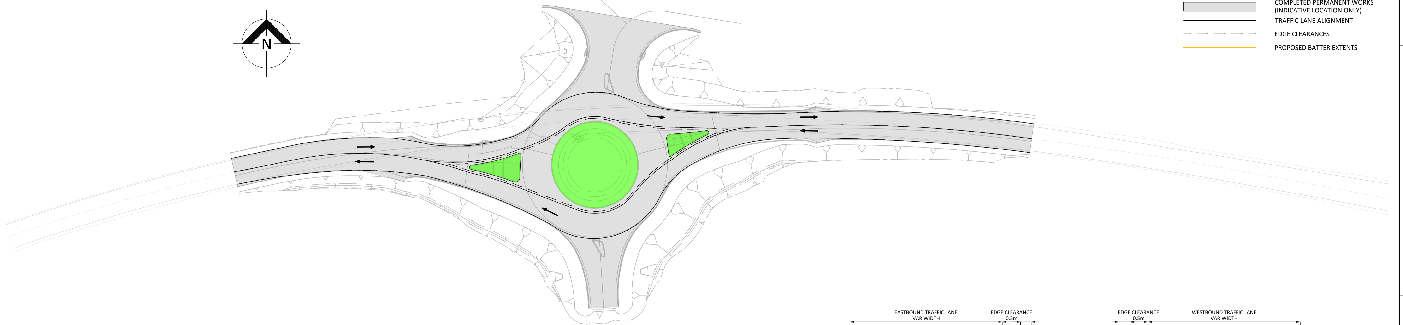
LAYOUT PLAN - TRAFFIC PATH SCALE 1:500
