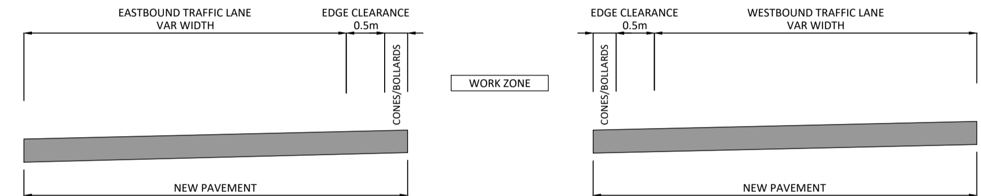
TYPICAL SECTION - TRAFFIC MANAGEMENT STAGE 5 NTS
