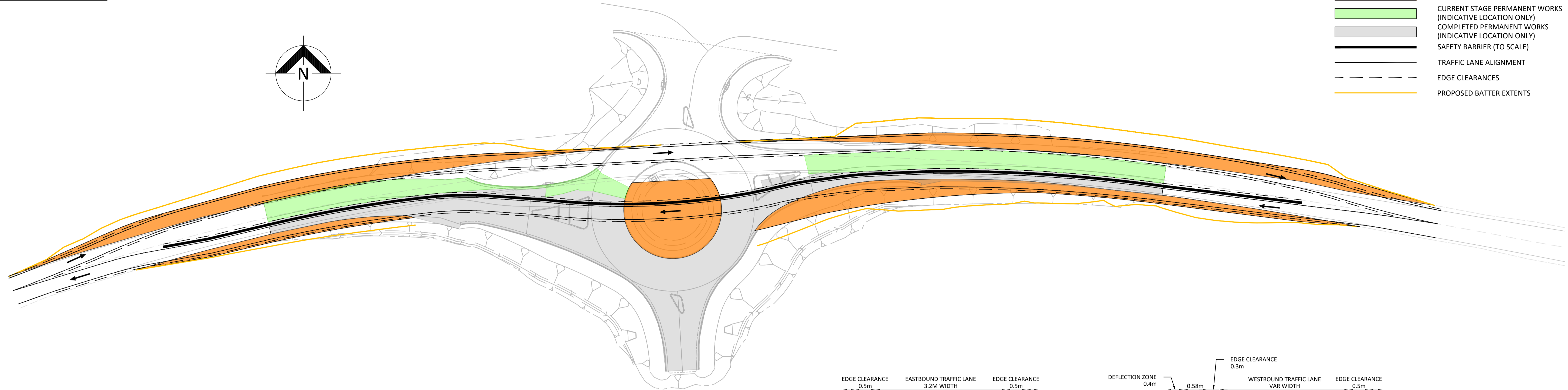
LAYOUT PLAN - TRAFFIC PATH SCALE 1:500
