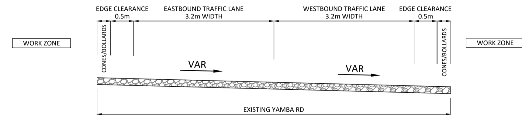
TYPICAL SECTION - TRAFFIC MANAGEMENT STAGE 1 NTS
