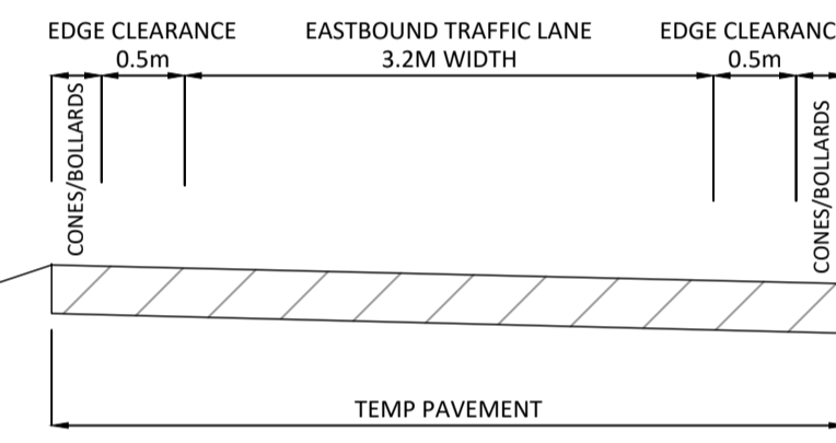
TYPICAL SECTION - TRAFFIC MANAGEMENT STAGE 3 NTS
