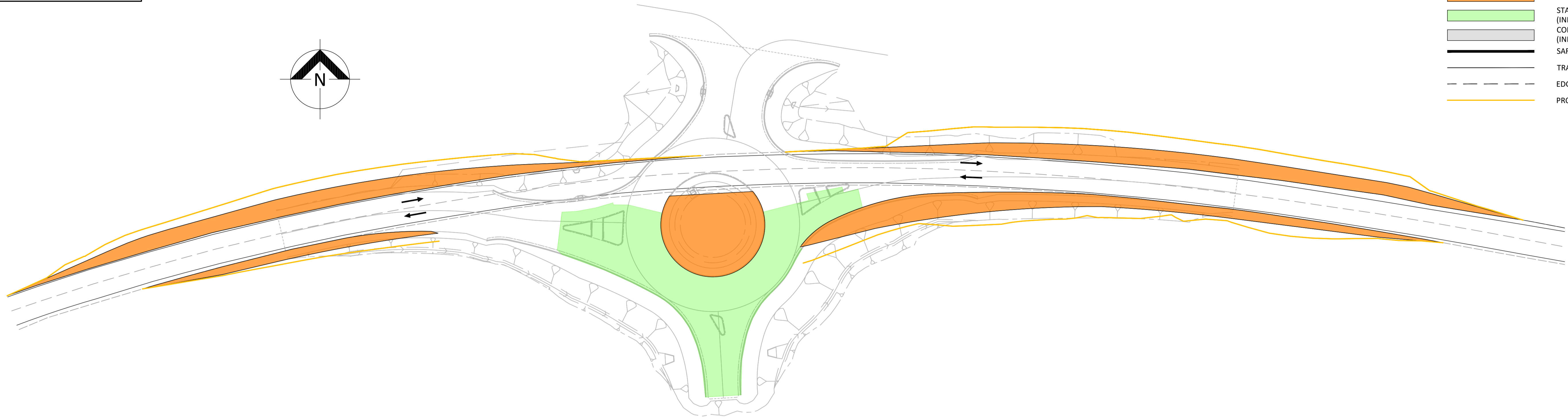
LAYOUT PLAN - TRAFFIC PATH SCALE 1:500
