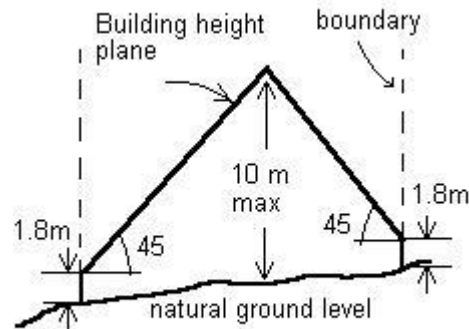
SLOPING SITE
